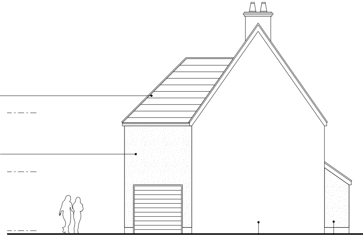
PROPOSED SIDE ELEVATION (DWELLING 7)
